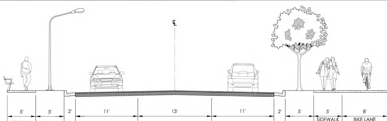
AKINS BLVD EXTENSION TYPICAL SECTION NTS
